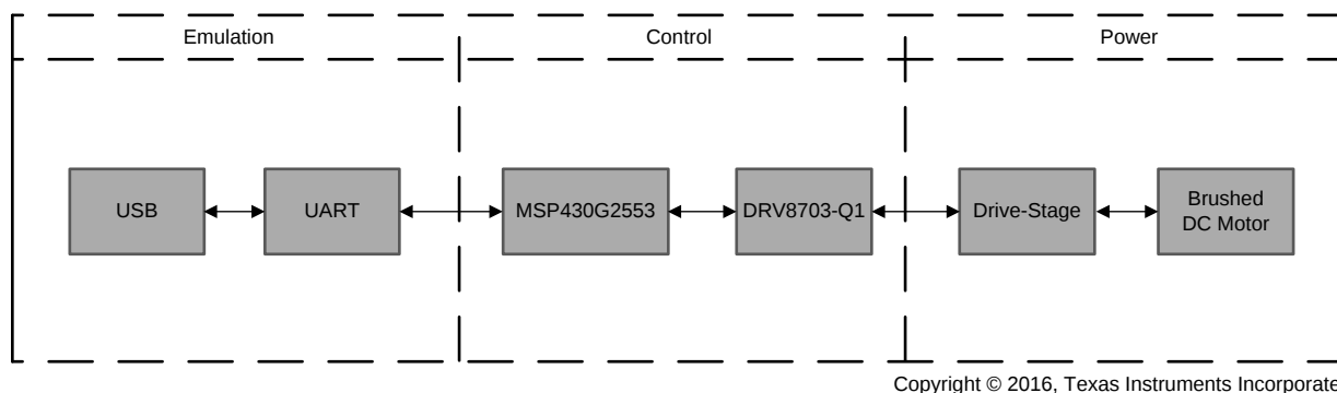
Figure 2. Block Diagram
