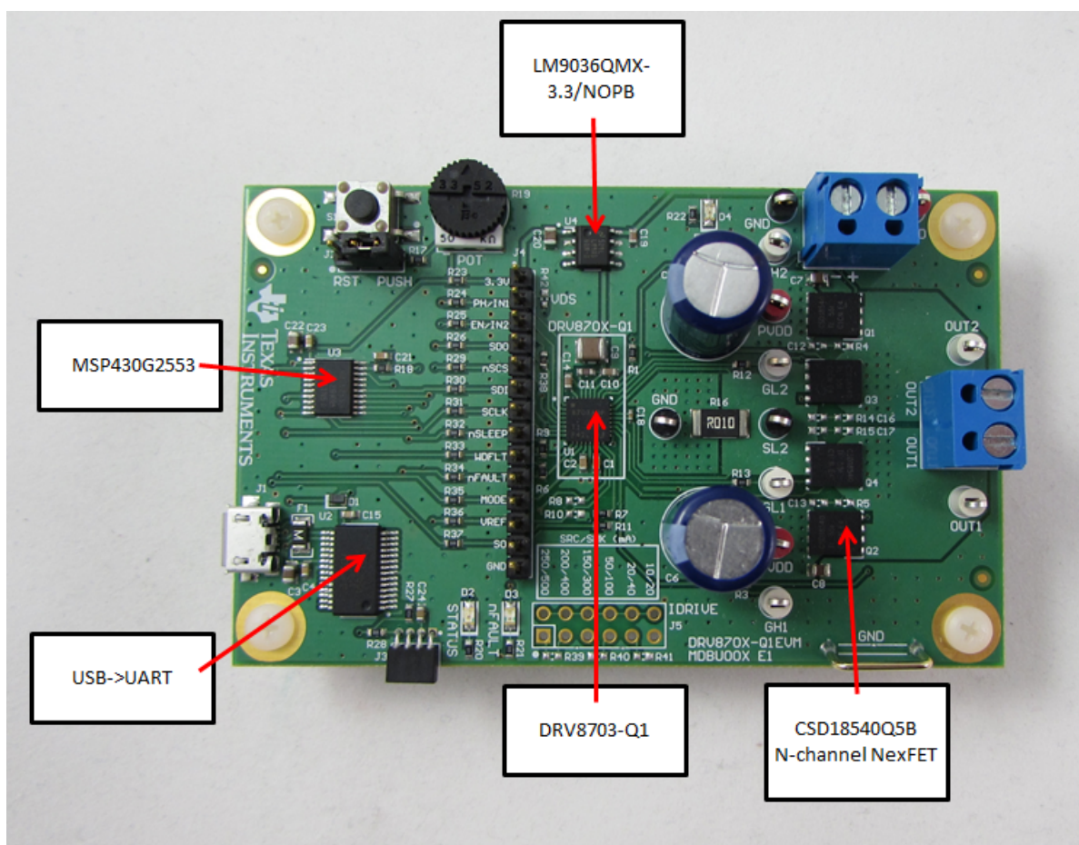
Figure 1. Board Components
