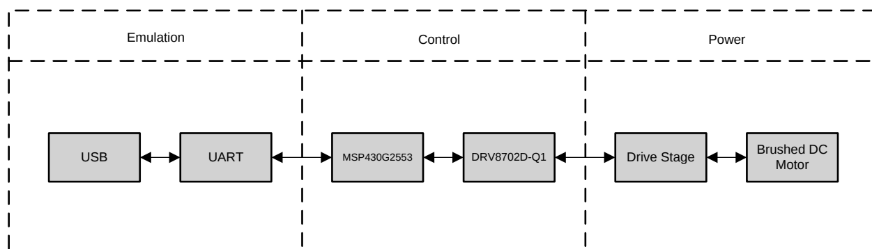
Figure 2. Block Diagram
