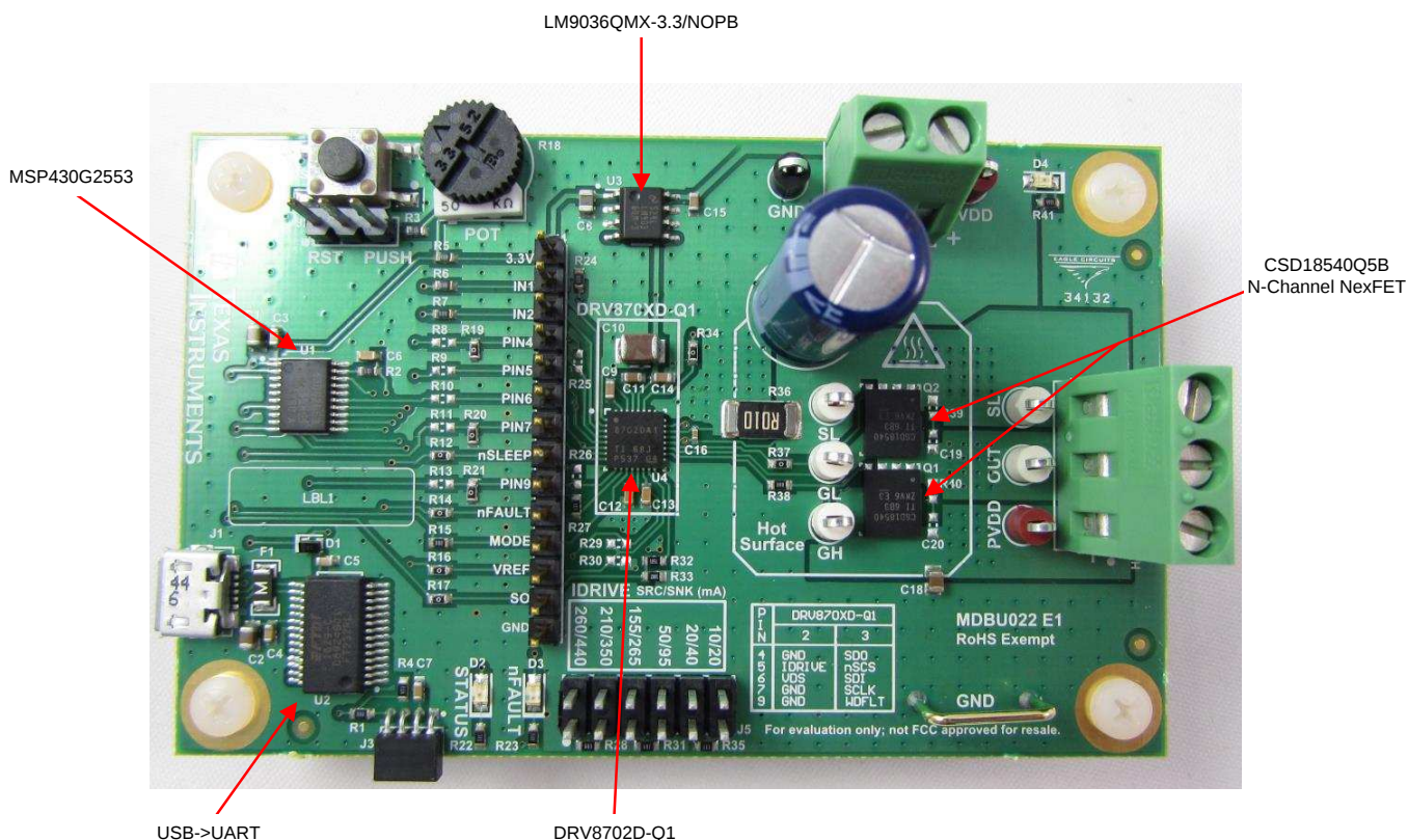
Figure 1. Board Components
