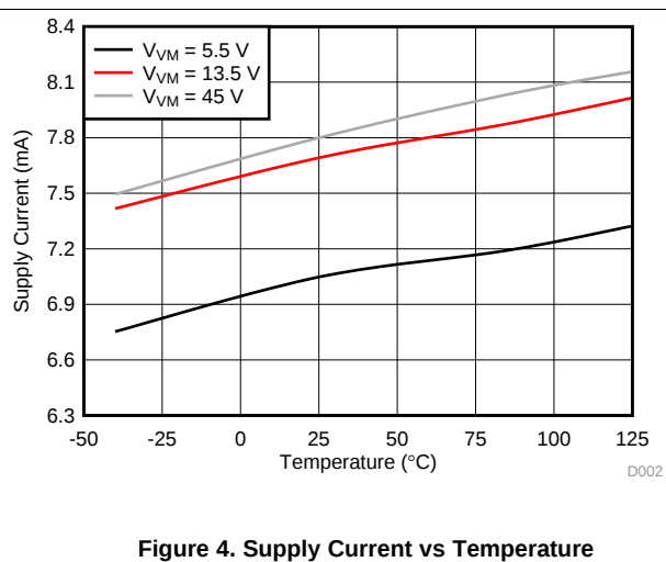
Figure 4. Supply Current vs Temperature
