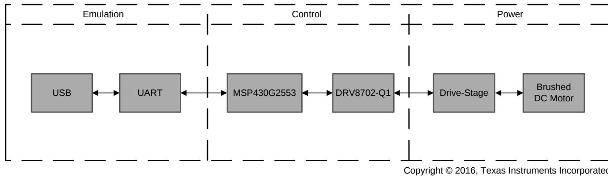
Figure 2. Block Diagram
