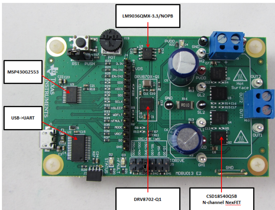
Figure 1. Board Components
