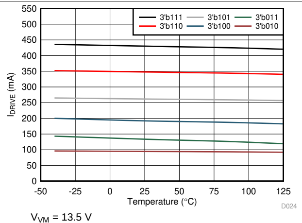
Figure 26. High-Side Sink Current
