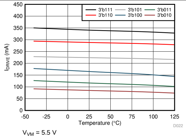
Figure 24. Low-Side Sink Current
