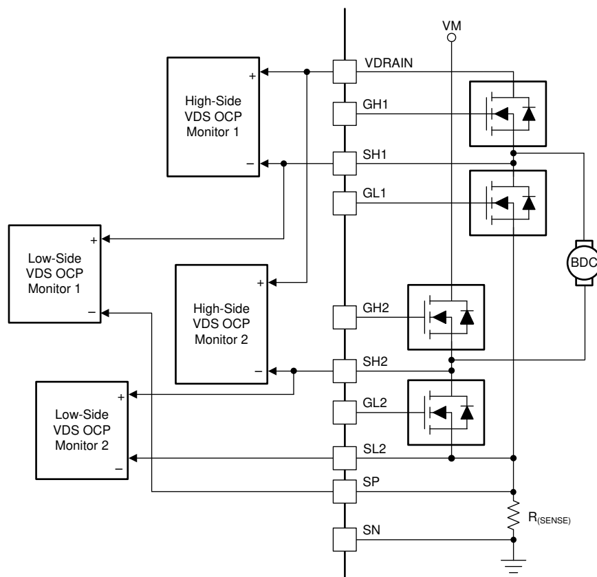
Figure 41. V_{\text{DS(OC)}} Block Diagram
