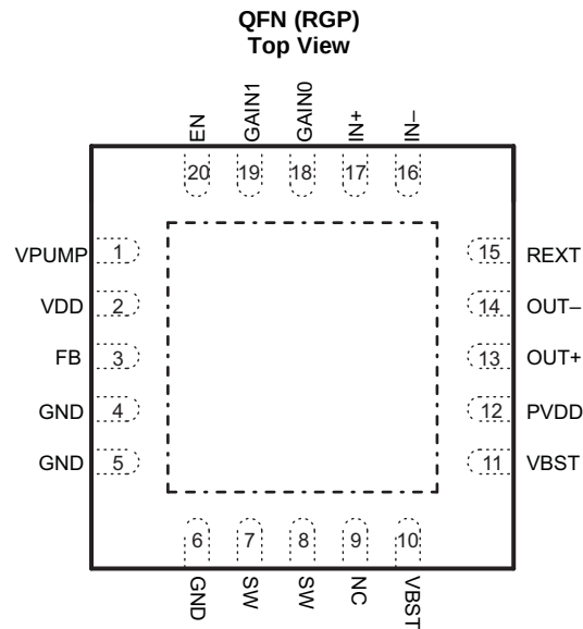
Pin Functions
