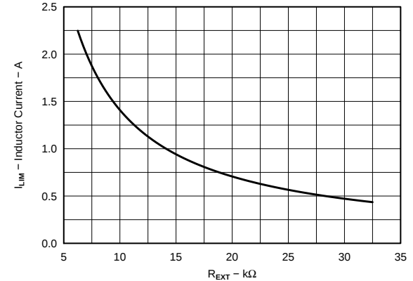
Figure 12. I_{LIM} vs R_{EXT}
