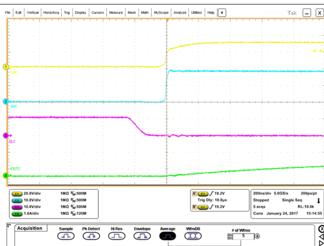
Figure 61. IDRIVE 260 to 520-mA Setting Positive Current
