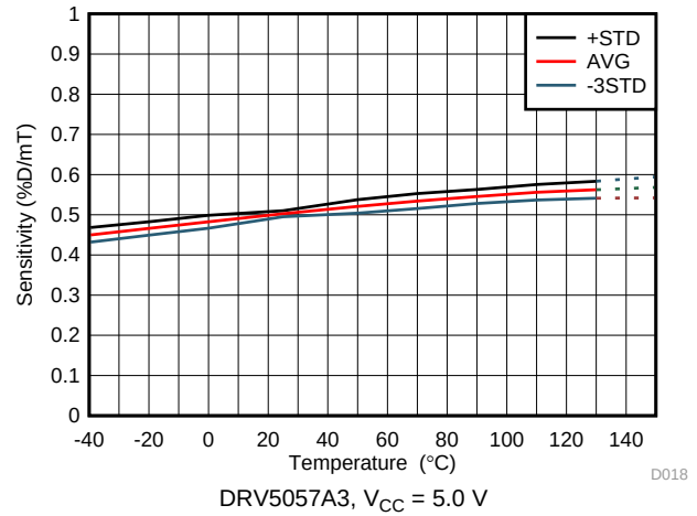
Figure 8. Sensitivity vs Temperature
