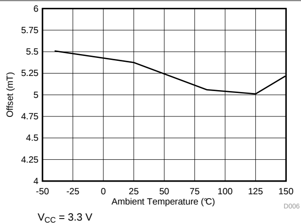
Figure 10. DRV5033-Q1AJ, Offset vs Temperature
