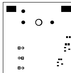
Figure 3. DRV5032-SOLAR-EVM Top Solder Mask
