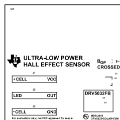
Figure 2. DRV5032-SOLAR-EVM Top Overlay
