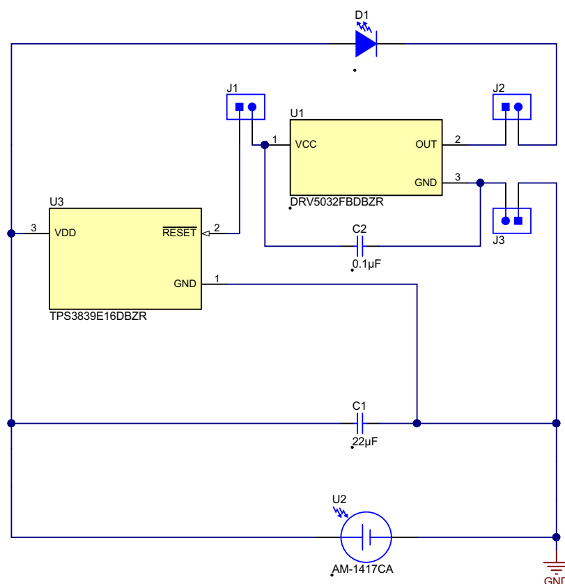
Figure 1. DRV5032-SOLAR-EVM Schematic
