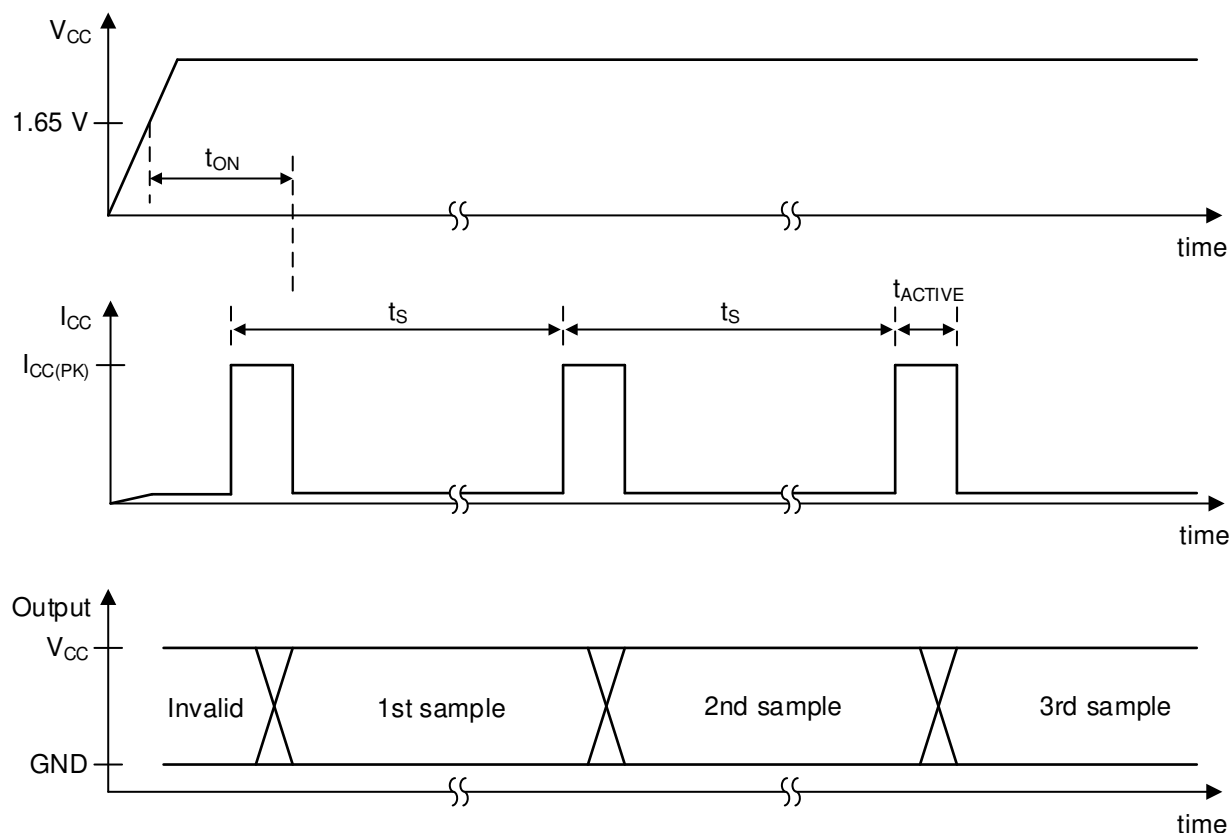
Figure 20. Timing Diagram
