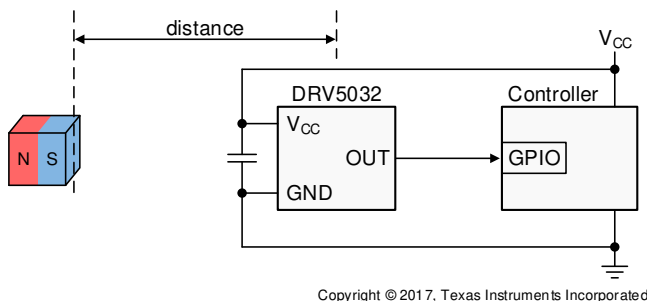
Typical Schematic
