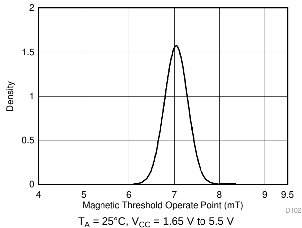
Figure 11. AJ Version B_{OP} Probability Density Function
