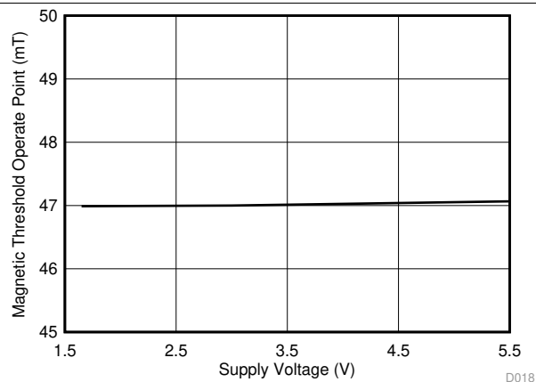
Figure 9. ZE Version |B_{OP}| vs V_{CC}
