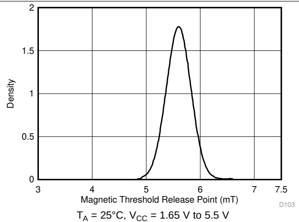
Figure 12. AJ Version B_{RP} Probability Density Function
