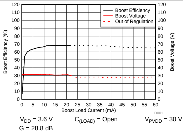
Figure 1. Load Current vs Boost Efficiency (%) and Voltage (V) at V_{PVDD} = 30\text{ V}
