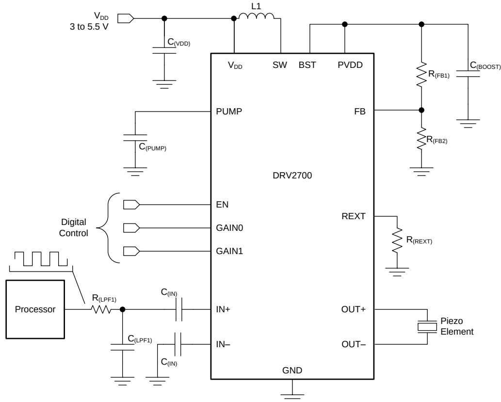
Figure 33. Filtered AC Coupled Single-Ended PWM Input
