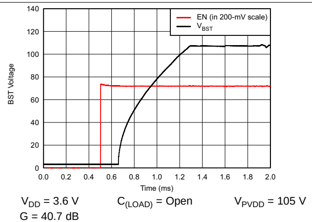
Figure 6. Boost Voltage Startup
