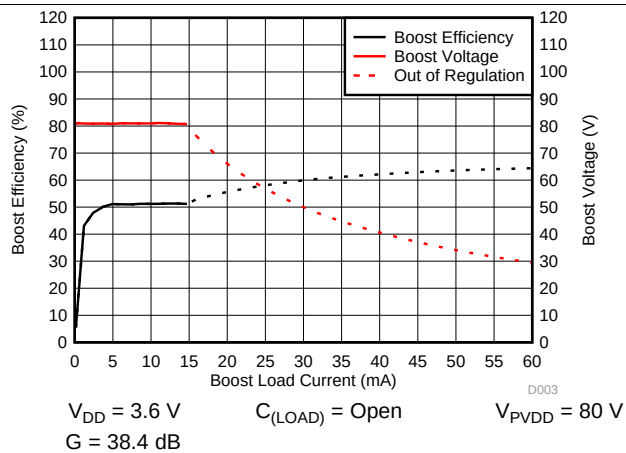
Figure 3. Load Current vs Boost Efficiency (%) and Voltage (V) at V_{PVDD} = 80\text{ V}
