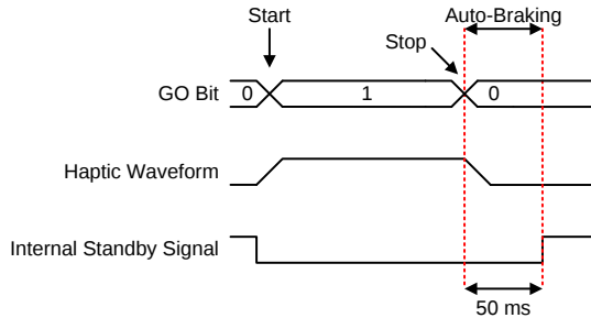
图 40. Playback Start and stop Trigger (Internal GO bit) (RTP or Waveform Sequencer)
