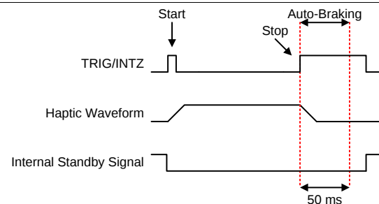
图 45. Trigger-Pulse Behavior when TRIG/INTZ Pin Left High (RTP or Waveform Sequencer)
