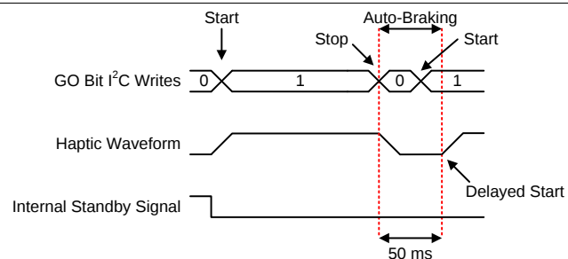
图 44. GO bit Trigger with Delayed Start (RTP or Waveform Sequencer)
