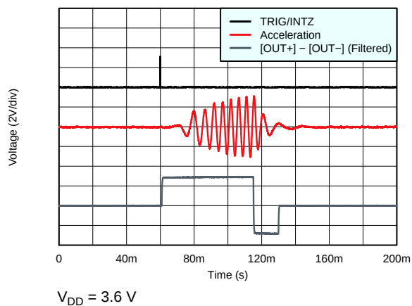
Figure 5. ERM Click (Open-Loop) with External Pulse-Trigger
