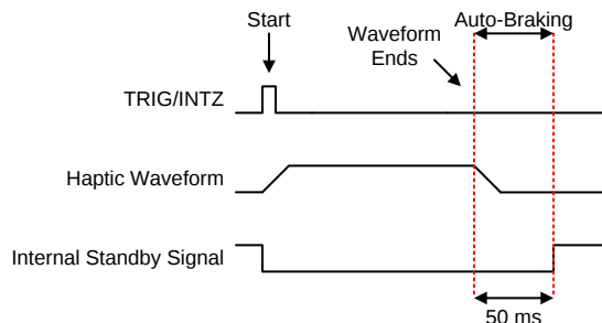
Figure 34. Waveform Sequencer with Trigger-Pulse
