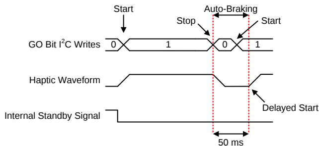
Figure 44. GO bit Trigger with Delayed Start (RTP or Waveform Sequencer)
