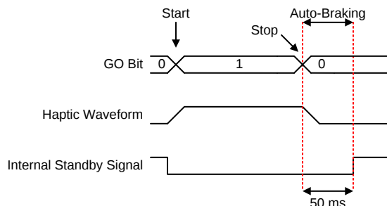
Figure 40. Playback Start and stop Trigger (Internal GO bit) (RTP or Waveform Sequencer)
