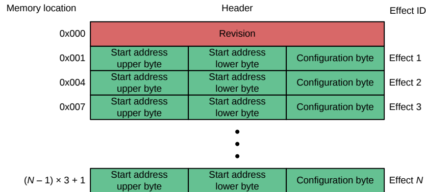
Figure 30. Header Structure
