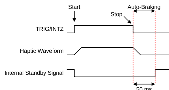
Figure 39. Playback Start and stop Trigger (Level)(RTP or Waveform Sequencer)
