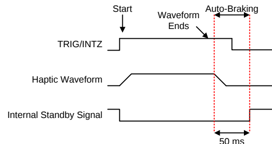
Figure 35. Waveform Sequencer with Trigger-Level
