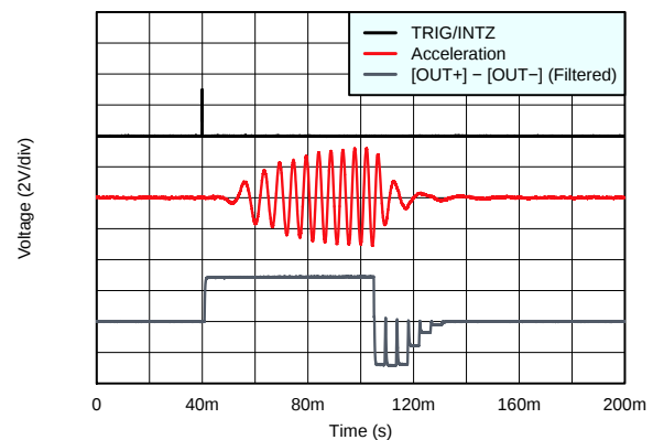
Figure 103. ERM Open-Loop Drive with Automatic Brake
