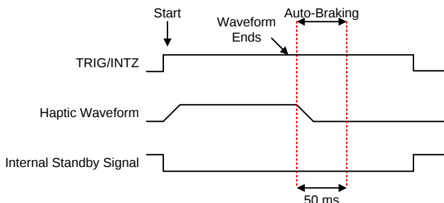
Figure 36. Waveform Sequencer with Trigger-Level Behavior when TRIG/INTZ Pin Left High
