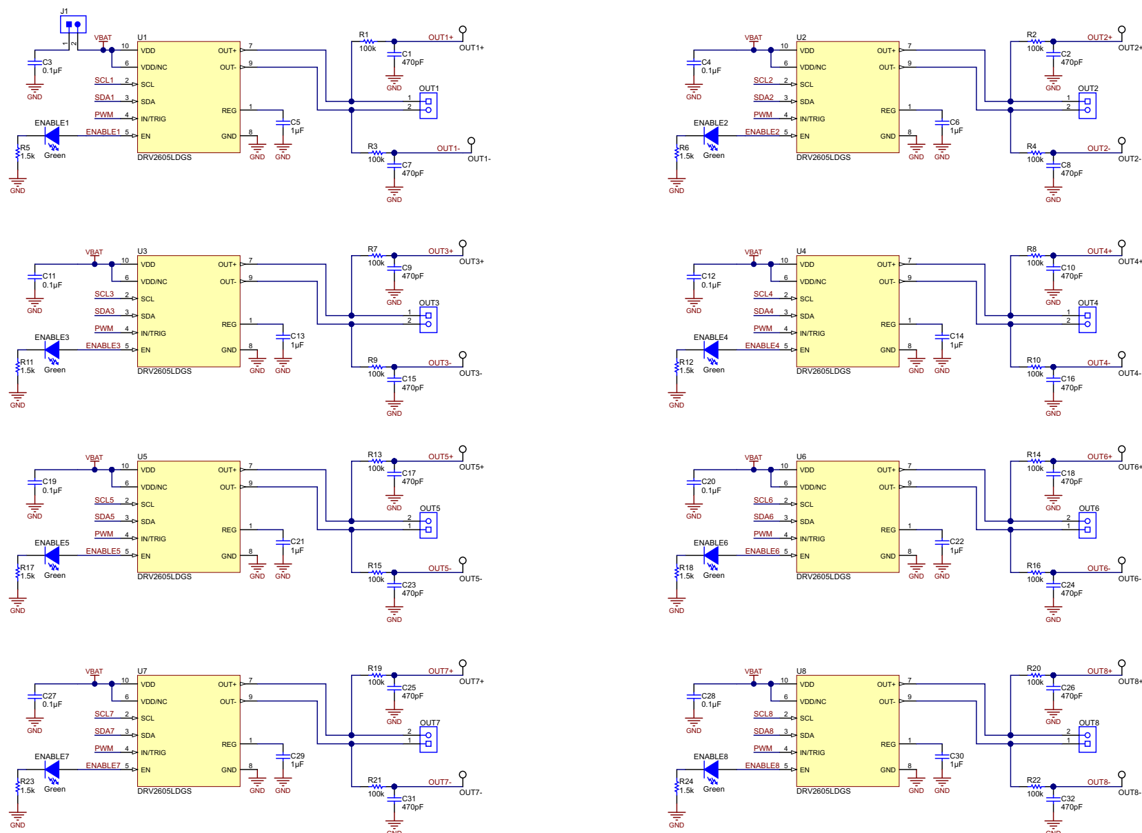
Figure 21. Schematic Page 1
