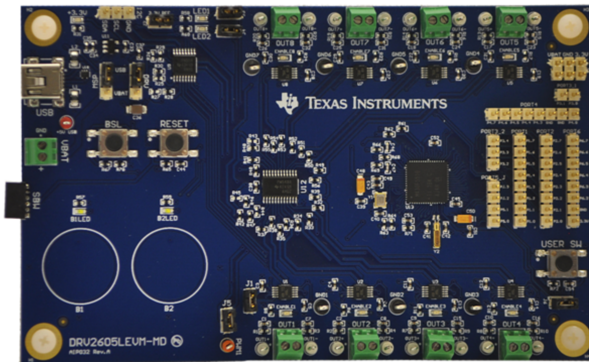
Figure 1. DRV2605LEVMD
