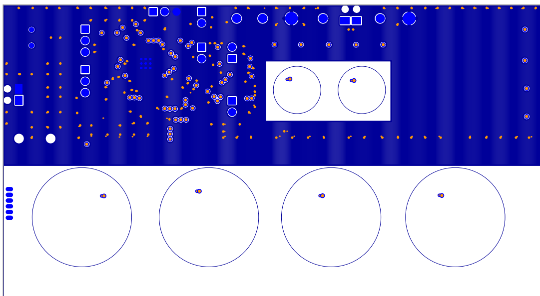
Figure 27. Layer 2 Copper
