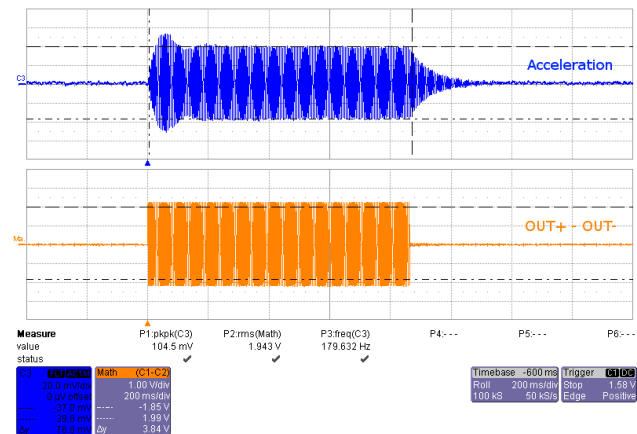
Figure 10. LRA Auto-Resonance OFF Waveform (Button 2)
