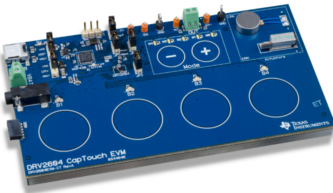
Figure 1. DRV2604EVM-CT Board
