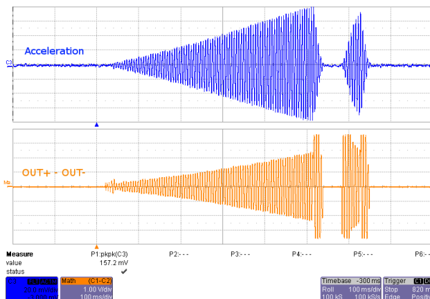
Figure 4. LRA Ramp-Up and Click Waveform (Button 2)
