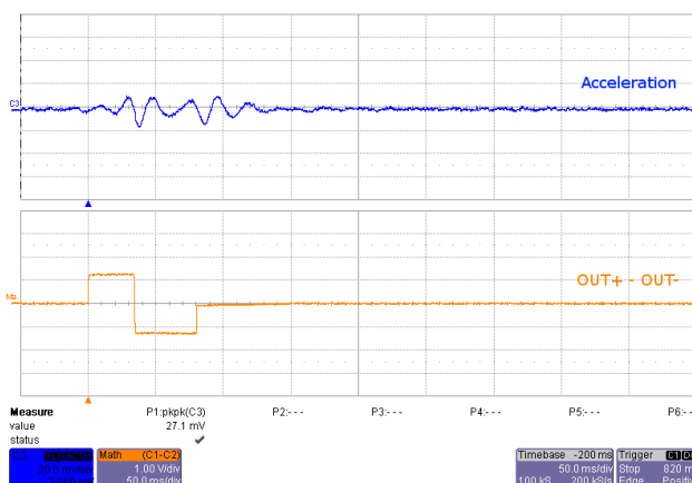
Figure 6. ERM Open-Loop Click Waveform (Button 4)
