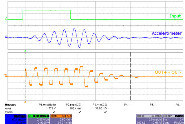
Figure 21. DRV2604 Filtered Waveform
