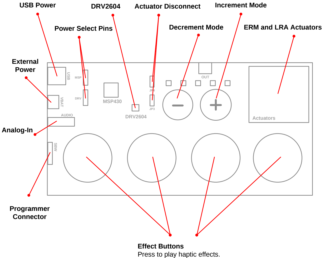
Figure 2. Board Diagram
