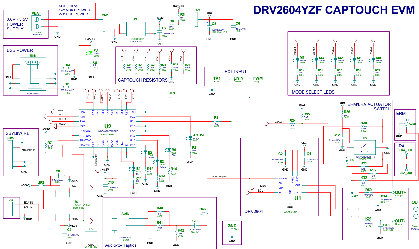
Figure 24. DRV2604EVM-CT Schematic
