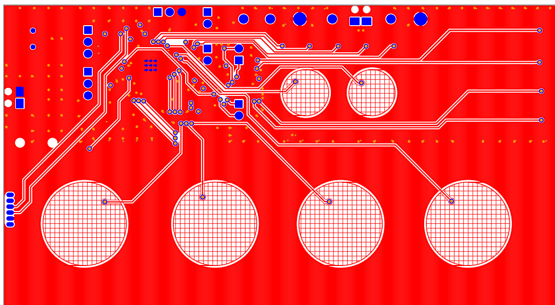
Figure 29. Bottom Copper
