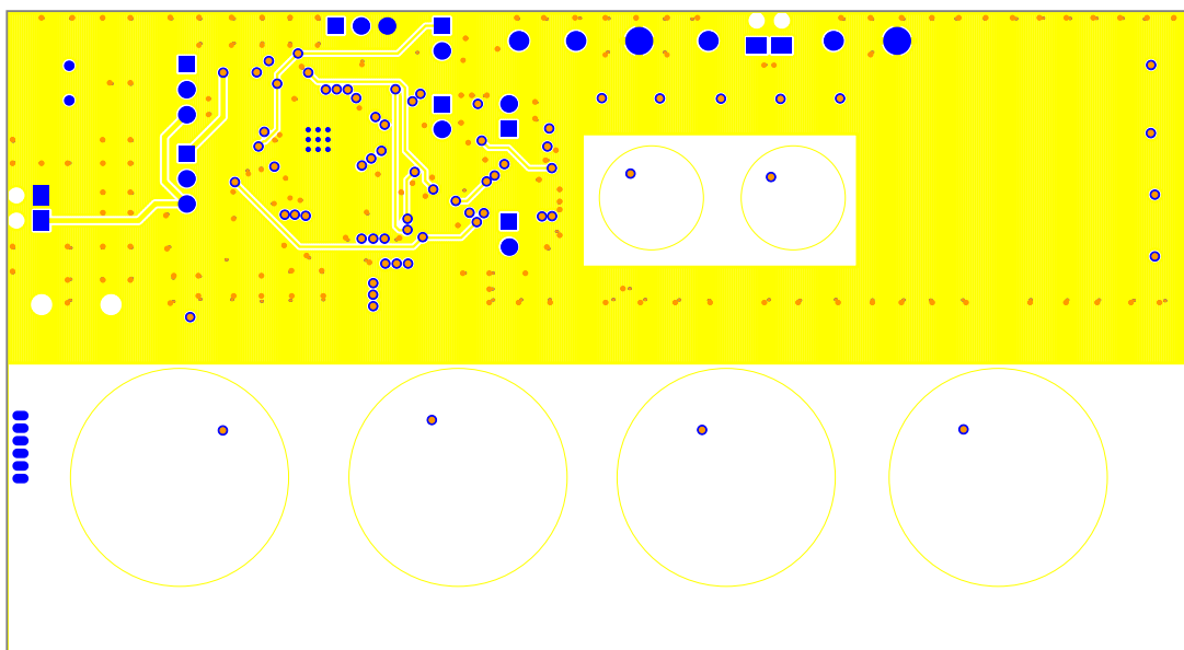
Figure 28. Layer 3 Copper
