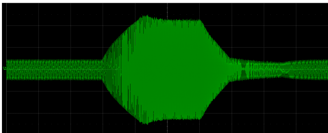
Figure 36. Phase Current With Speed Control Waveform
