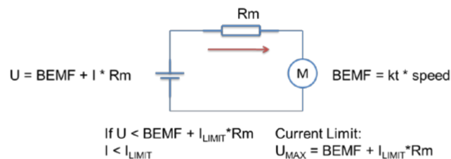
Figure 13. Current Limit
