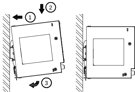
Fig. 6.1 Mounting
