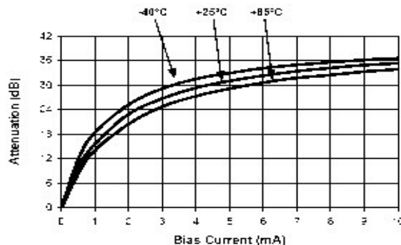
Attenuation vs. Bias Current Frequency = 1000 MHz
