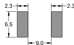
PCB PAD LAYOUT (REF.)
