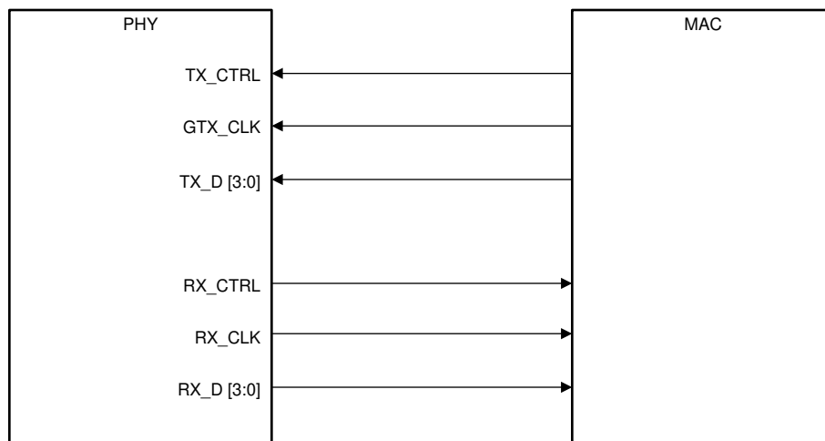
Figure 16. RGMII Connections
