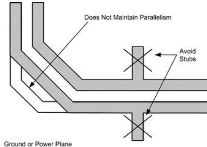
Figure 39. Avoiding Stubs in a Differential Signal Pair
