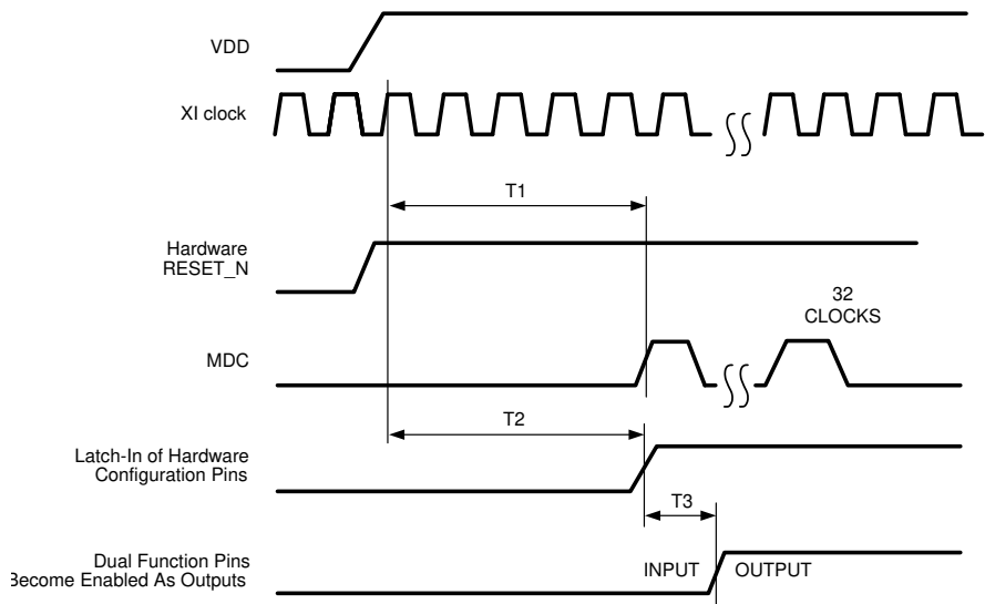
Figure 1. Power-Up Timing
