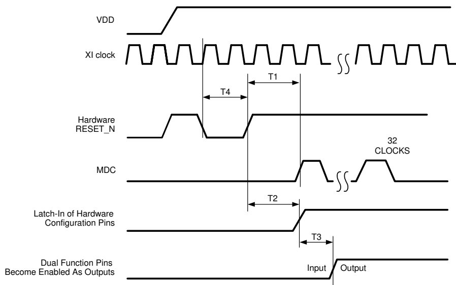
Figure 2. Reset Timing
