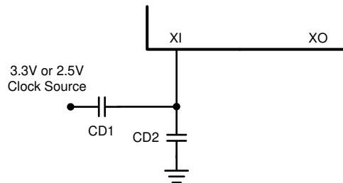
Figure 32. Clock Divider
