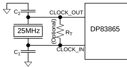
Crystal option circuit
