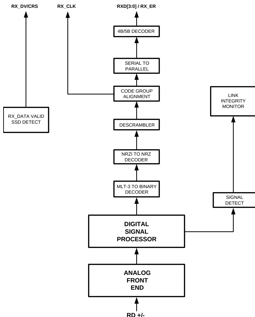
Figure 8-1. 10/100 Mb/s Twisted Pair Interface
