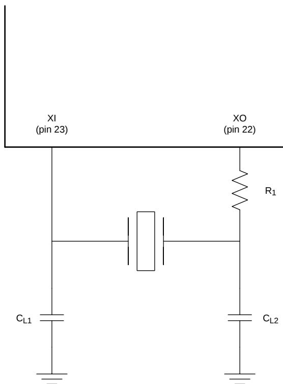
Figure 18. Crystal Oscillator Circuit
