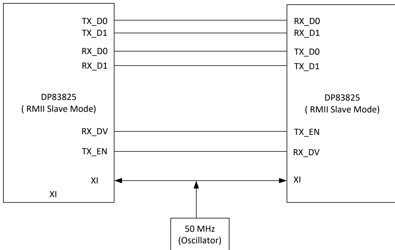
Figure 11. RMII Repeater Mode
