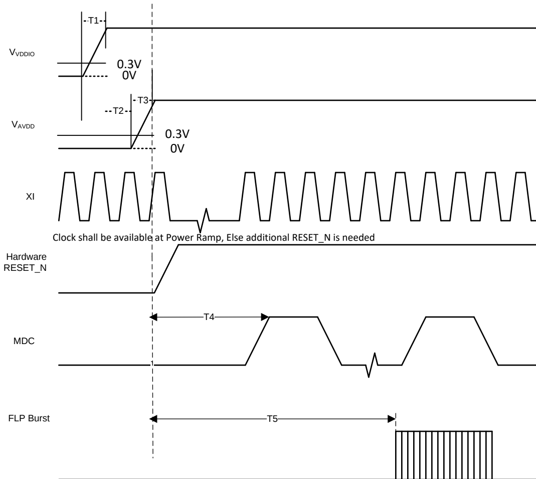
Figure 1. Power-Up Timing
