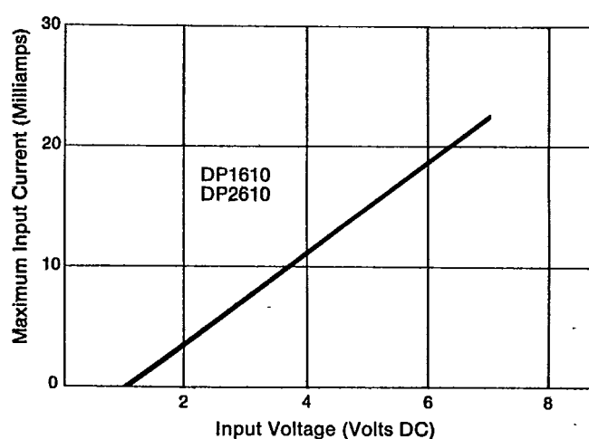
Figure 4. Input Characteristics (Voltage Controlled)
