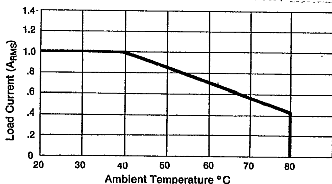
Figure 1. Derating Curve
