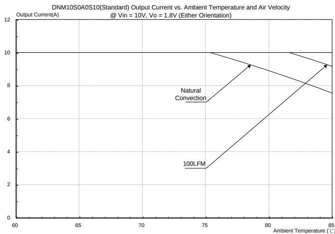
Figure 33: DNM10S0A0S10(Standard) Output current vs. ambient temperature and air velocity @ V_{in}=10V , V_o=1.8V (Either Orientation)
