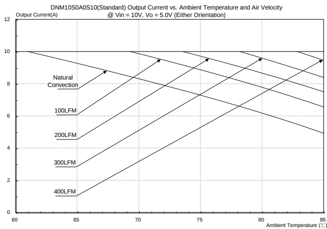
Figure 32: DNM10S0A0S10(Standard) Output current vs. ambient temperature and air velocity @ V_{in}=10V , V_o=5.0V (Either Orientation)
