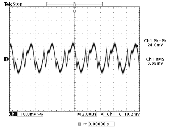
Figure 9: Output ripple & noise at 12Vin, 5.0V/10A out
