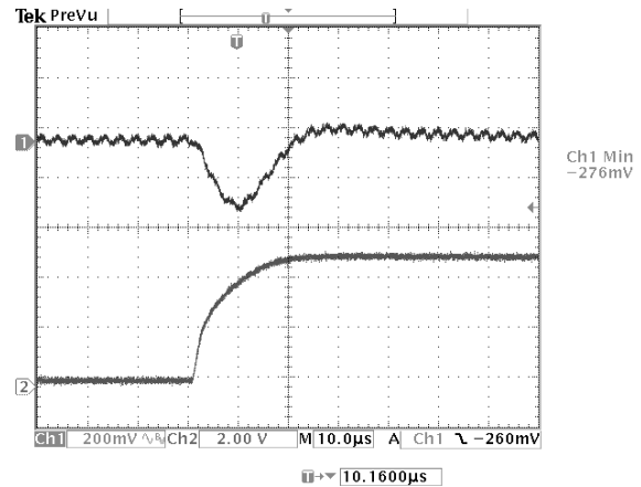
Figure 14: Typical transient response to step load change at 2.5A/\mu S from 50% to 100% of I_o , max at 12Vin, 5.0V out ( C_{out} = 1\mu F ceramic, 10\mu F tantalum)
