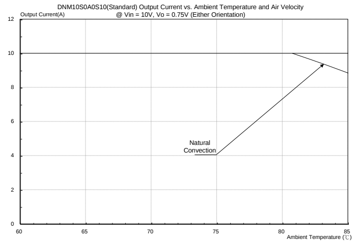
Figure 34: DNM10S0A0S10(Standard) Output current vs. ambient temperature and air velocity @ V_{in}=10V , V_o=0.75V (Either Orientation)
