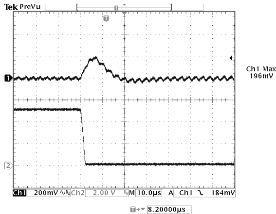
Figure 13: Typical transient response to step load change at 2.5A/\mu S from 100% to 50% of I_o , max at 12Vin, 5.0V out ( C_{out} = 1\mu F ceramic, 10\mu F tantalum)
