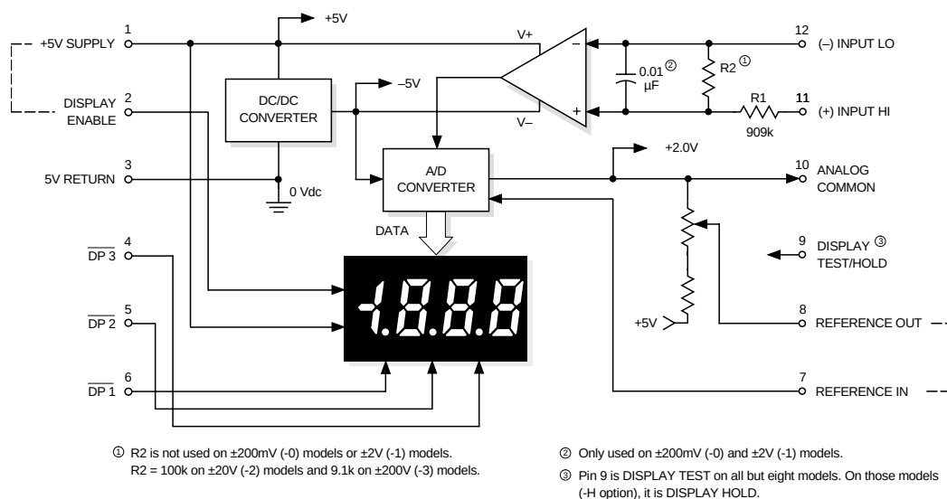
Figure 1. DMS-20PC Series Simplified Schematic
