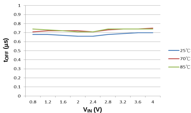
t_{OFF} vs. V_{IN} ( V_{BIAS}=5.5V )
