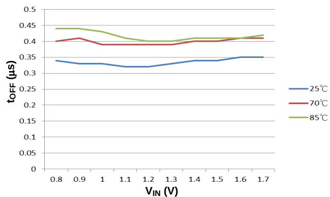
t_{OFF} vs. V_{IN} ( V_{BIAS}=3.2V )
