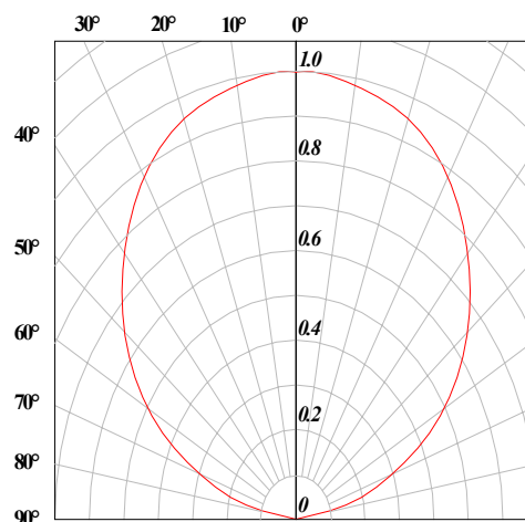
Radiation Pattern
