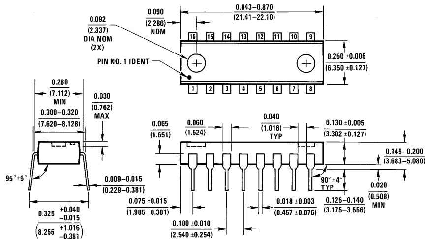
Order Number DM2502CM or DM2503CN NS Package Number N16A
