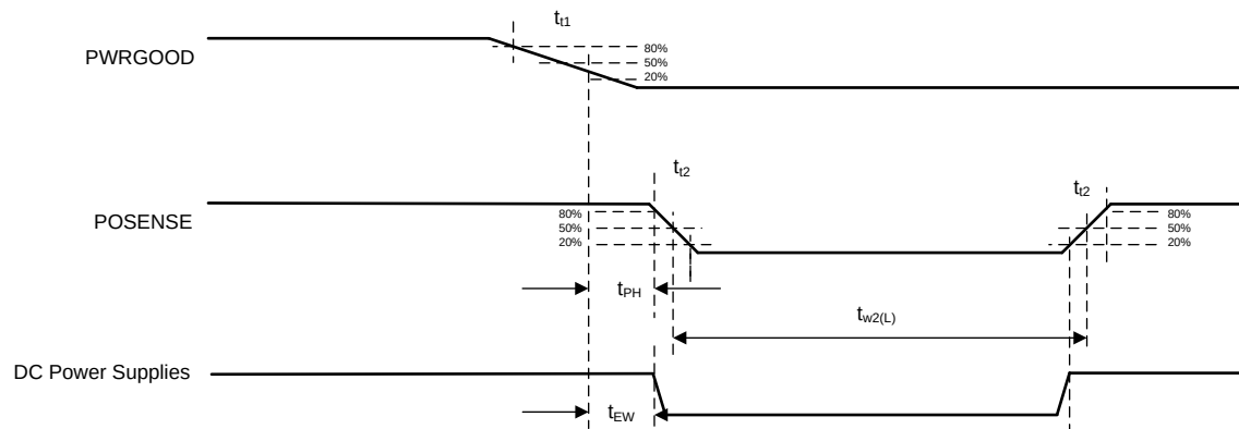
Figure 3. Power Down
