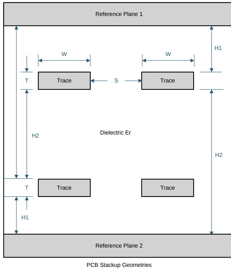
Figure 15. PCB Stackup Geometries
