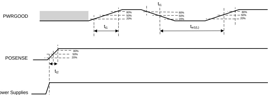
Figure 2. Power Up
