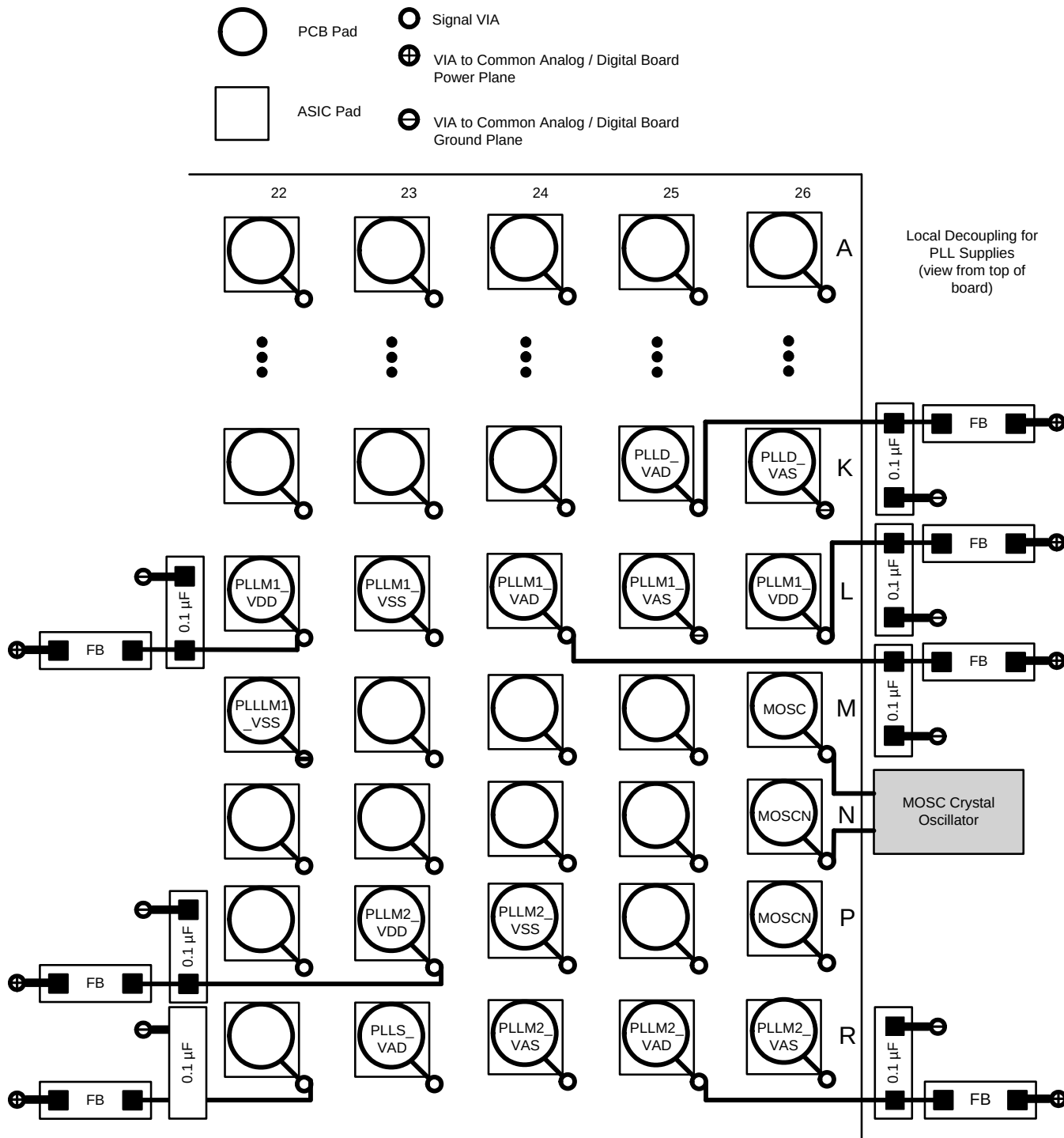
Figure 14. PLL Filter Layout
