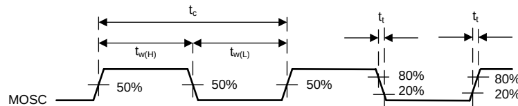
Figure 1. System Oscillators
