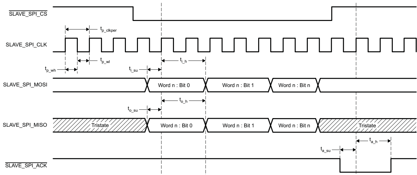
Figure 5. SPI Timing
