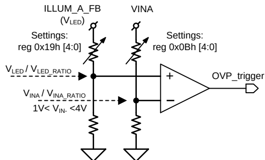
Figure 11. Ratio Metric OVP
