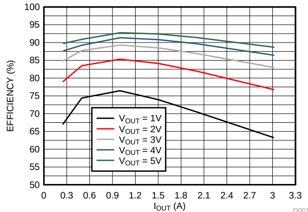
Figure 18. Buck Converter Efficiency vs I_{OUT} ( V_{IN} = 12\text{ V} )
