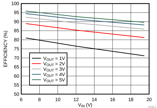
Figure 19. Buck Converter Efficiency vs V_{IN} ( I_{OUT} = 1\text{ A} ) Schematic
