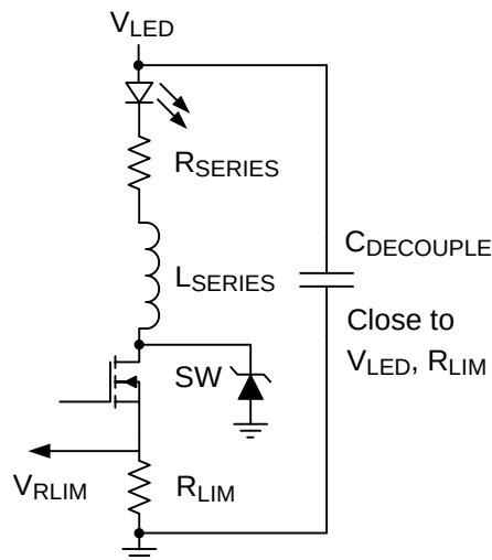
Figure 31. Parasitic Inductance ( L_{\text{series}} ) and Resistance ( R_{\text{series}} ) in Series with LED
