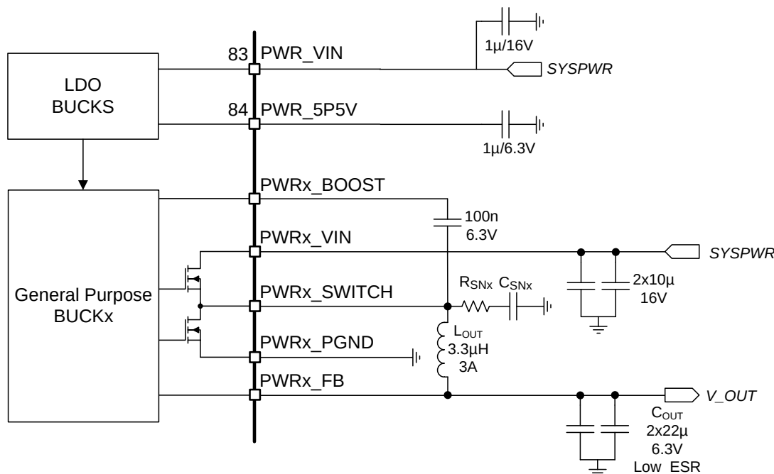
Figure 17. Buck Converter
