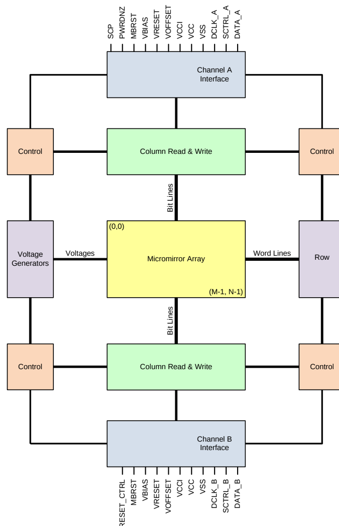
Figure 10. Functional Block Diagram
