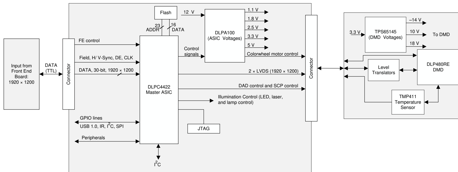
Figure 12. Typical WUXGA Application Diagram
