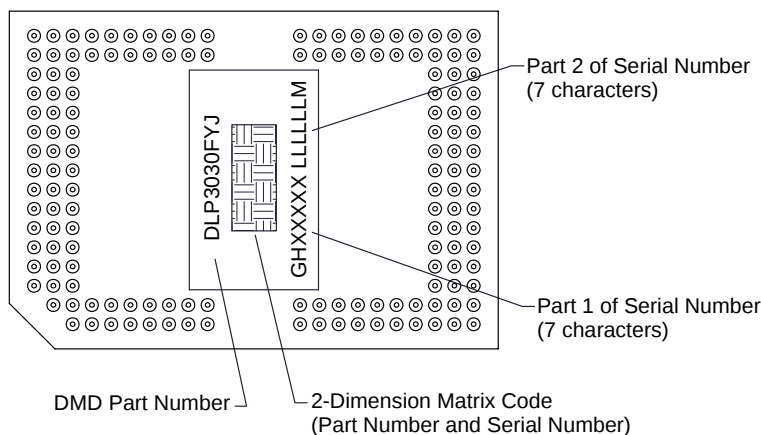
Figure 2. DMD Marking
