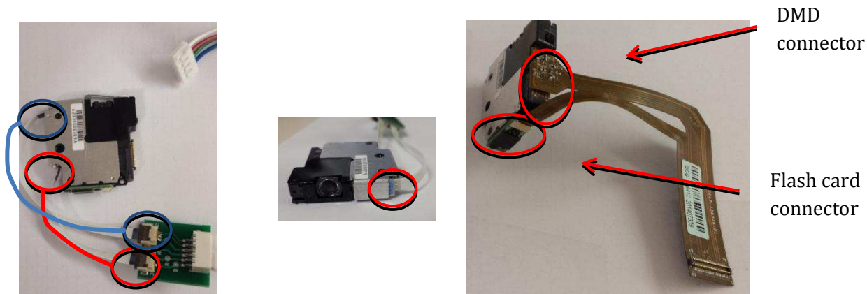
Figure 7. LED Connection and Flex Cable Connection
