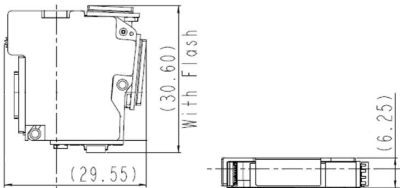
Figure 3. Dimensions of Optical Engine
