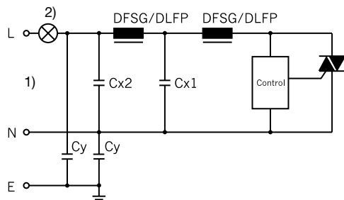
Interference suppression with resistive load, 2-phase
