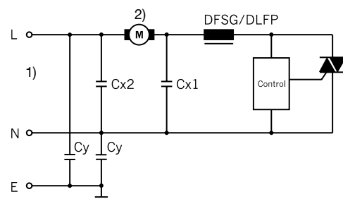
Interference suppression with inductive load
