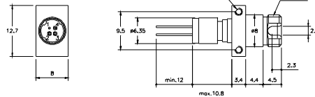
FC Receptacle (Board Mount)
