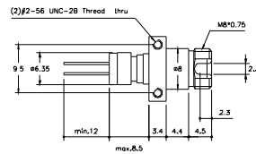
FC Receptacle (Board Mount)
