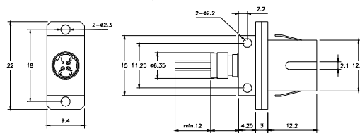
SC Receptacle (Board Mount)
