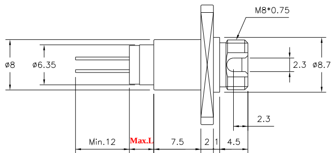
SC RECEPTACLE (BOARD MOUNT) (DL-55XXX-1625-SBS)
