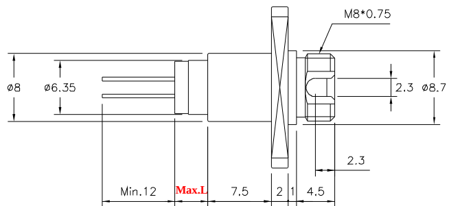
SC RECEPTACLE (BOARD MOUNT) (DL-55XXX-1490-SBX)
