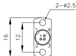
Vertical Flange
