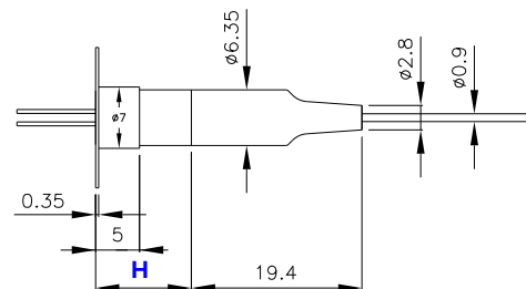
Vertical Flange
