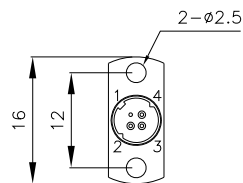
Vertical Flange
