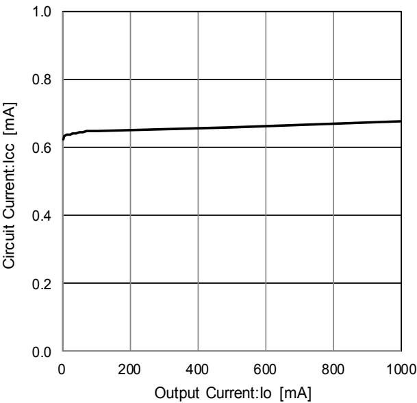
Figure 43. Circuit Current
