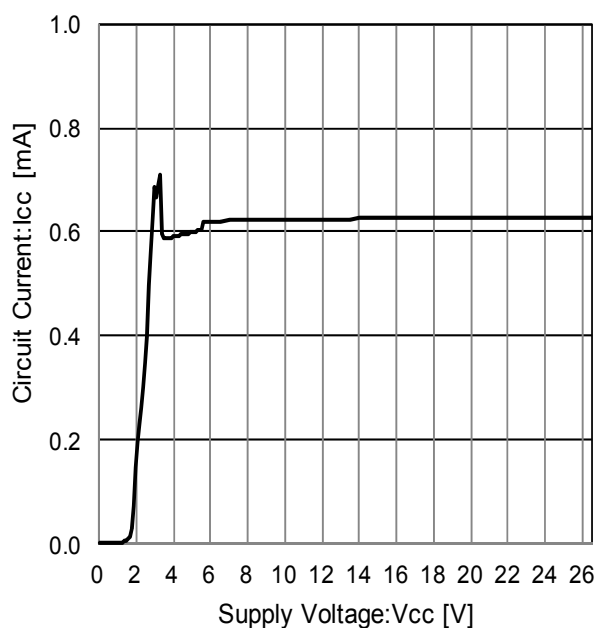
Figure 24. Circuit Current
