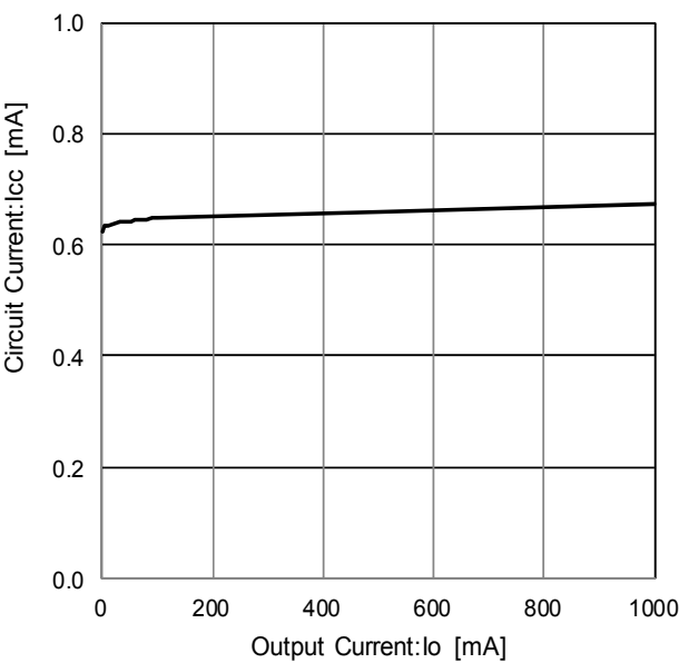
Figure 67. Circuit Current
