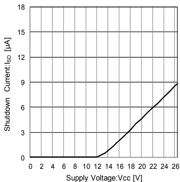
Figure 48. Shutdown Current
