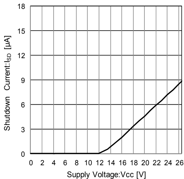
Figure 13. Shutdown Current
