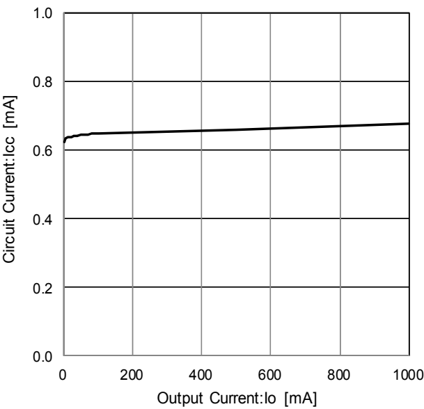
Figure 55. Circuit Current
