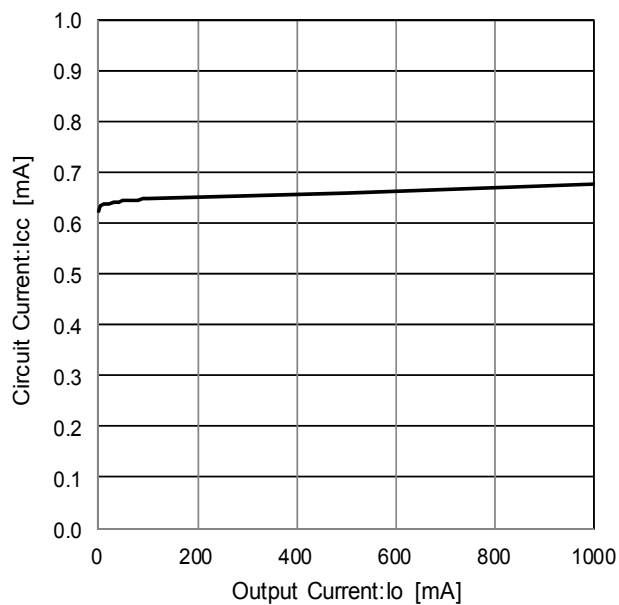
Figure 31. Circuit Current
