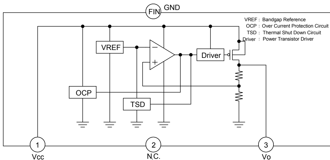
Figure 9. Block diagrams BDxxFC0FP (Output Voltage Fixed Type, without Shutdown SW)
