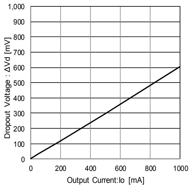
Figure 52. Dropout Voltage ( V_{cc}=V_o \times 0.95V )
