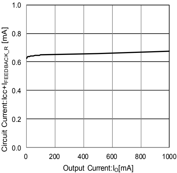
Figure 20. Circuit Current ( I_O = 0\text{mA} \rightarrow 1000\text{ mA} ) ( I_{FEEDBACK\_R} \approx 75\mu\text{A} )
