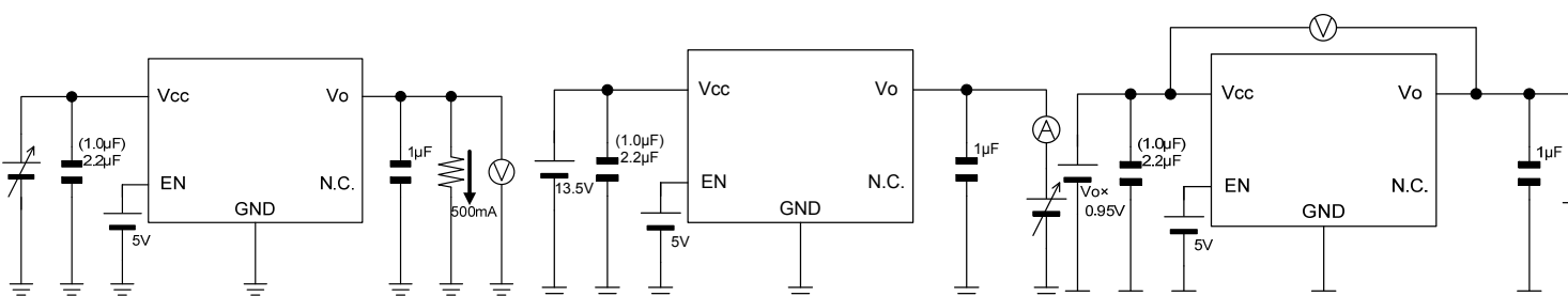
Measurement setup for Figure 27, 38, 50 and 62
