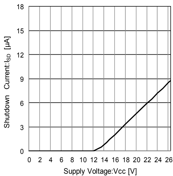
Figure 25. Shutdown Current
