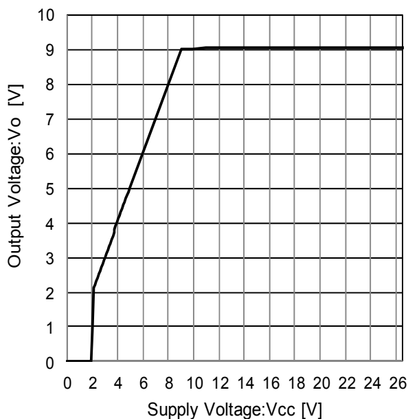
Figure 61. Line Regulation ( I_o=0\text{mA} )
