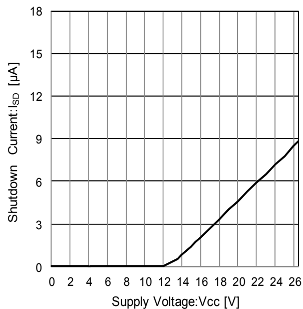
Figure 60. Shutdown Current
