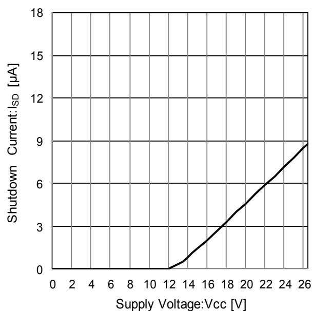
Figure 36. Shutdown Current
