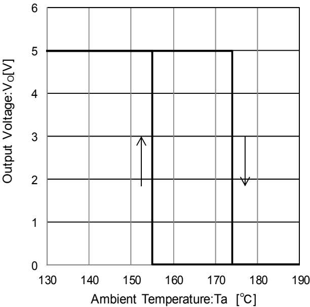
Figure 23. Thermal Shutdown Circuit Characteristic
