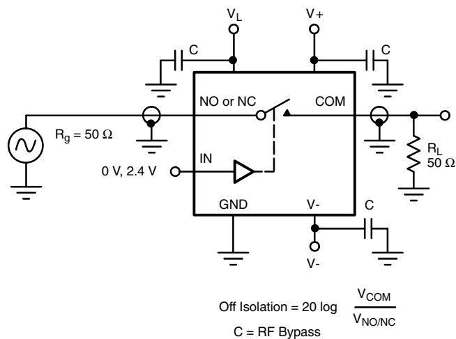
Figure 7. Off Isolation
