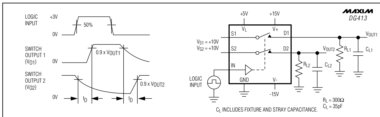
Figure 3. DG413 Break-Before-Make
