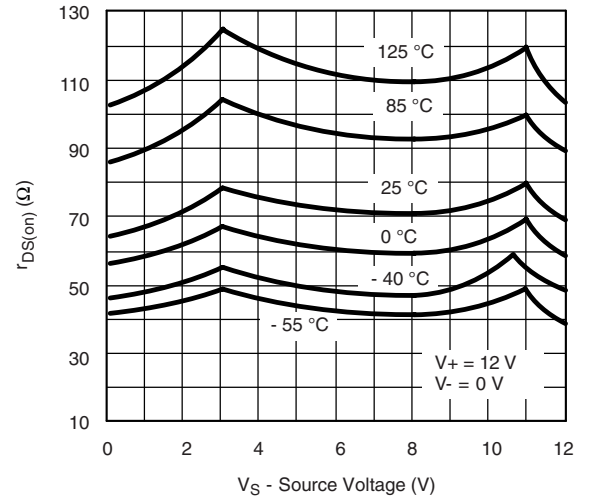
r_{DS(on)} vs. V_S and Temperature (Single Supply)
